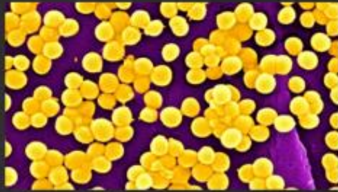
Staphylococcus aureus
