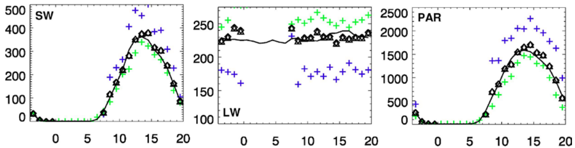
Fig. 7: Radiative fluxes (SW, \text{W/m}^2 , left; LW, \text{W/m}^2 , center and PAR, \mu\text{E/m}^2/\text{s} ) at Ice station Belgica: All skies (black solid lines), clear skies (blue crosses), and cloud skies (green crosses). Weighted means using the relative number of cloud hours (black diamonds) and cloudiness (black crosses) are shown. Data gaps reflect the lack of visual cloudiness observations during night time.
