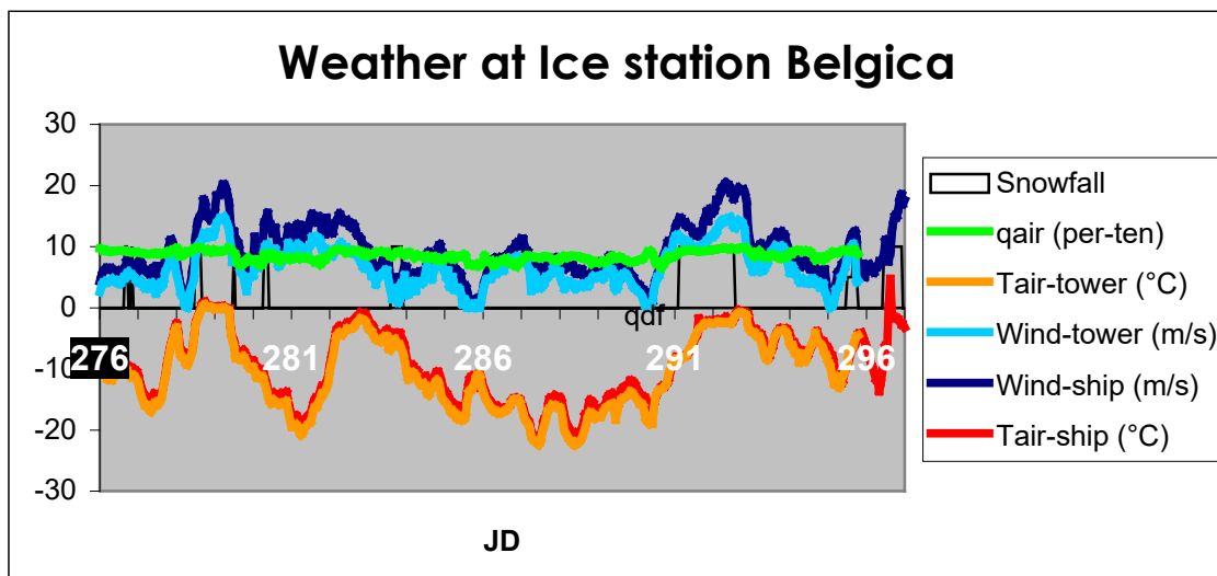
Fig. 3: Wind, temperature from SHIP and TOWER data sets recorded during ISB (blue and red curves). VISUAL Snow fall index (0 : no snow falling, 1: snow falling) is also plotted. Finally, the TOWER relative humidity (in 10ths) is also drawn.
