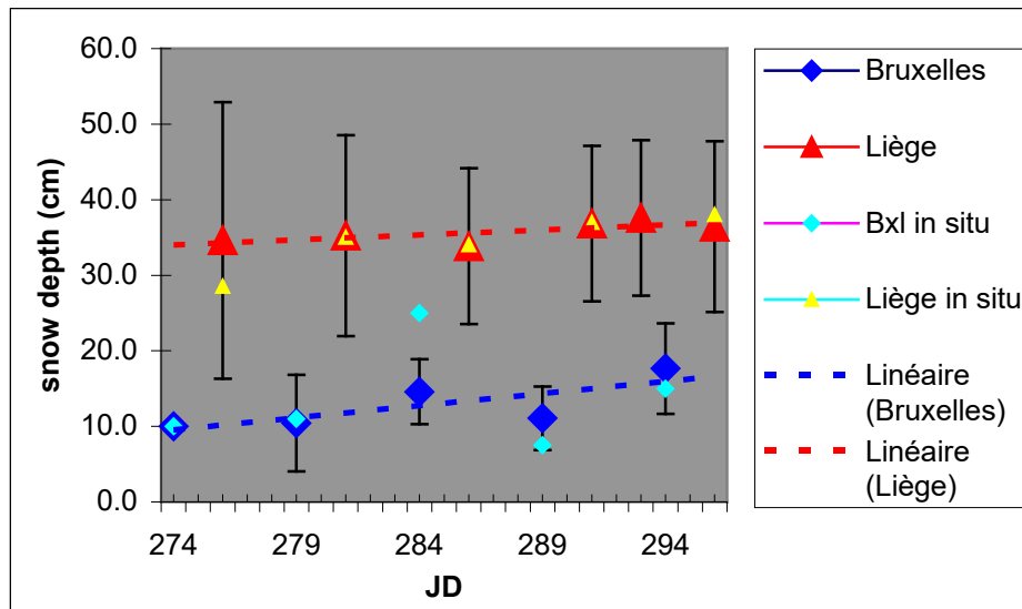
Fig. 9: Average snow depth along the 26 albedo line measurements made at each visit at Brussels (deep blue) and Liège (red). Trends and error bars are also depicted. The small blue diamonds and yellow triangles indicate the point snow measurement made at the BB subsite.
