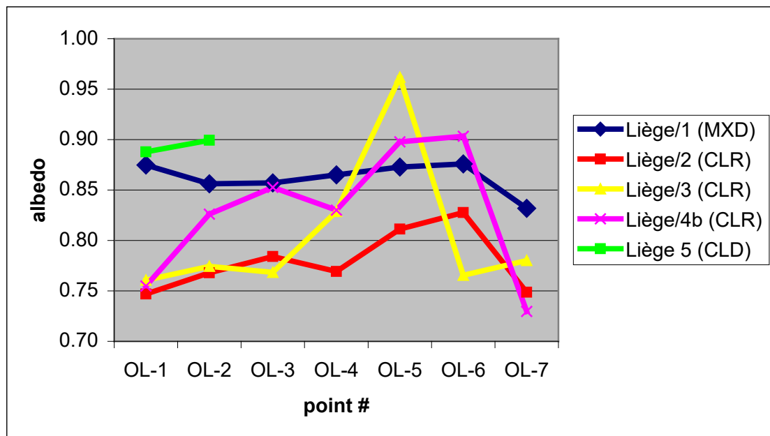
Fig. 12 : Same as Fig.11, but for Liège site
