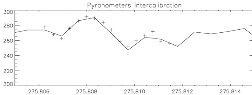
Fig. 6: Incoming SW (W/m 2 ) radiation measured by INSITU (crosses) and SHIP(solid line) pyranometers held side by side on the top of the ship's mast. X values are decimal julian days.
