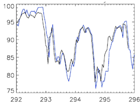
Fig. 4 : Relative humidity recorded by the SHIP (dark) and the TOWER (light) hygrometers between JD 292 and 296.
