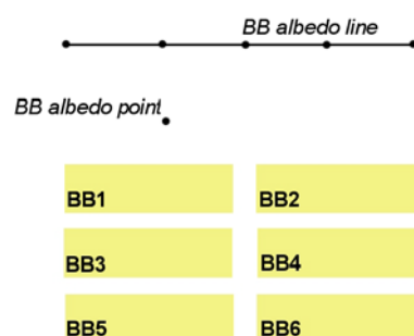
Fig. 8 : Brussels and Liège Sites spatial repartition.
