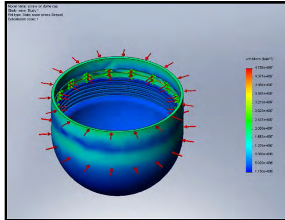
Figure 9: FEA of Components
