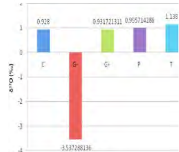
Figure 2C. Mean \delta^{18}\text{O} values of the ice type found in Figure 2A.
