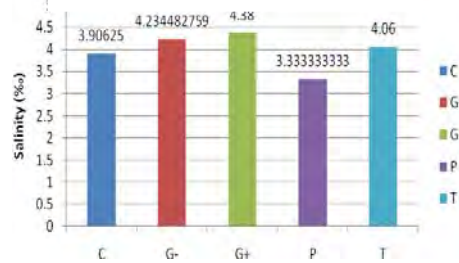
Figure 4B. Mean salinity values of the ice types present in the Figure 4A.
