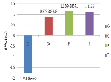
Figure 5C. Mean δ 18 O values of the ice type found in Figure 5A.
