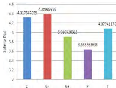
Figure 2B. Mean salinity values of the ice types present in the Figure 2A.
