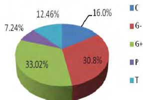
Overall Ice Type Concentrations
